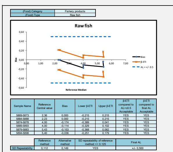
Figure 2. Accuracy profiles ( \beta = 80\% , AL = 0.5)
